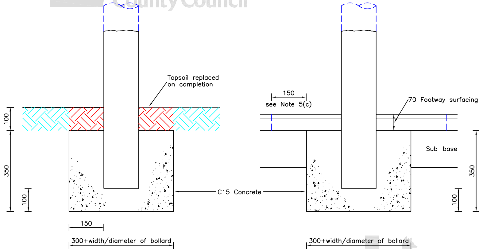
BOLLARD IN VERGE
